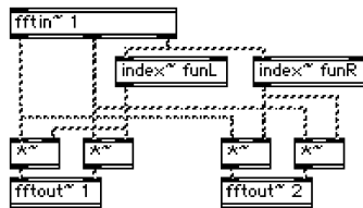
Figure 3: The pfft~ subpatch showing lookup in the two spatial information tables for stereo spectral spatialization.
